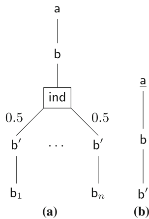
Fig. 14 A p-document (a) of \text{PrXML}_{b'}^{(\text{ind})} on which a v-insertion defined by single-path pattern (b) can result in exponential blowup
