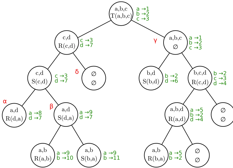
Fig. 2 Tree encoding of the relational instance from Example 1
