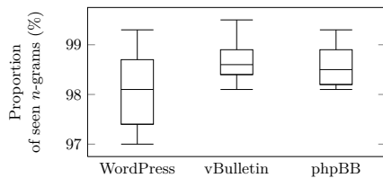
Fig. 4. Box chart of the proportion of seen n -grams for the three considered CMSs. We show in each case the minimum and maximum values (whiskers), first and third quartiles (box) and median (horizontal rule).
